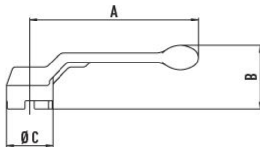
Art. 7010N Levier / Palanca TOTAL - DELTA - ROLLY - AIRY - KOSMOS
